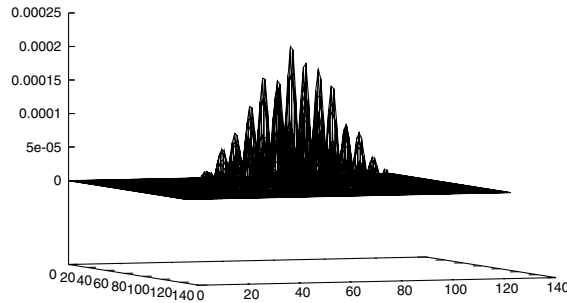
Fig. 2. Cross section of the charge density for the state at the top of the valence band (VBM). The wave-function is confined to the interior of the spherical CdSe quantum dot (which is centered in the middle of the box).
